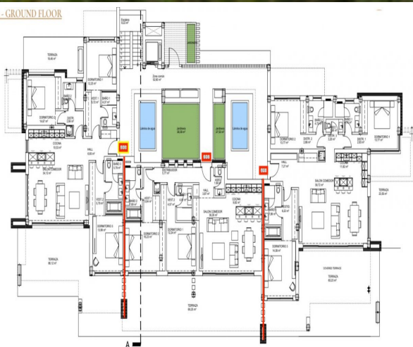
BLOCK 2 - GROUND FLOOR
